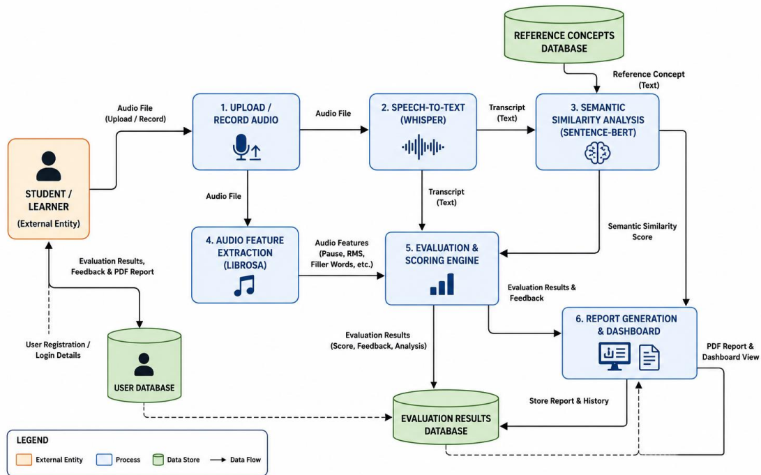
DATA FLOW DIAGRAM (DFD) – VOICE-BASED CONCEPT UNDERSTANDING ANALYSER (VBCUA)
